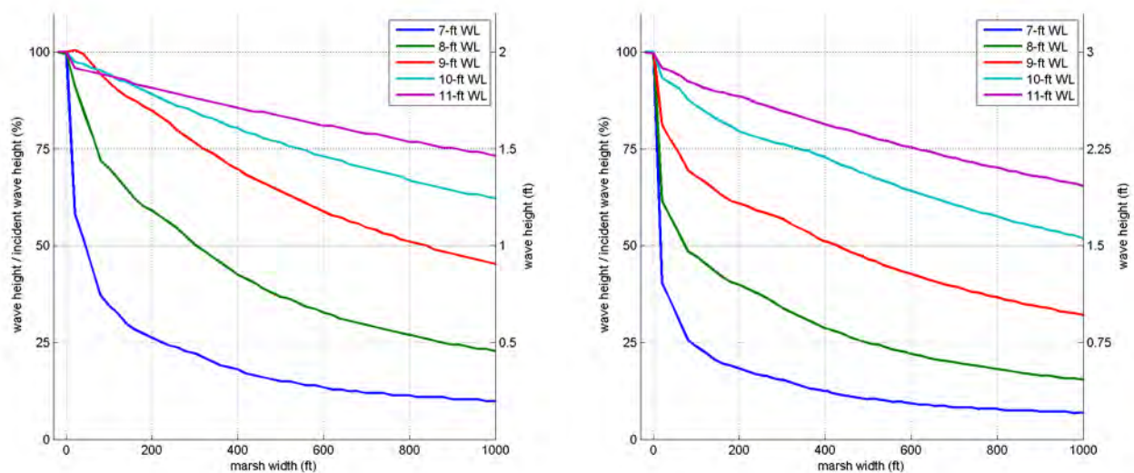
Figure 18. Predicted wave heights relative to incident wave height as a function of marsh width, from the WHAFIS model (see section 7). The incident wave height equals (a) 2 feet and (b) 3ft (BCDC 2013).
